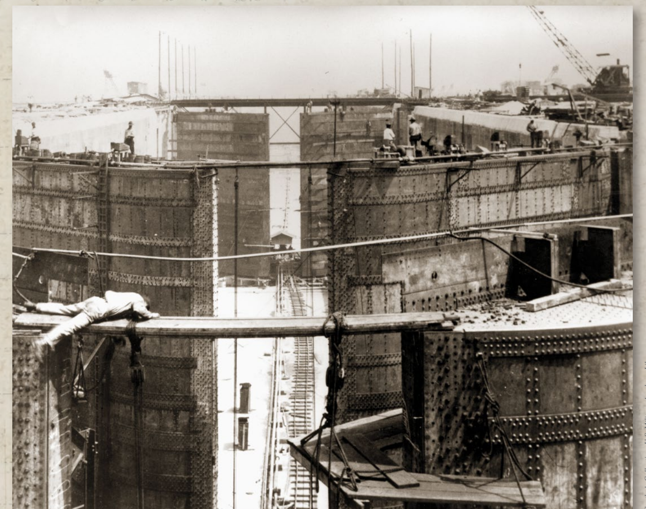
Gatun Lock Construction, Panama Canal, March 12, 1912
